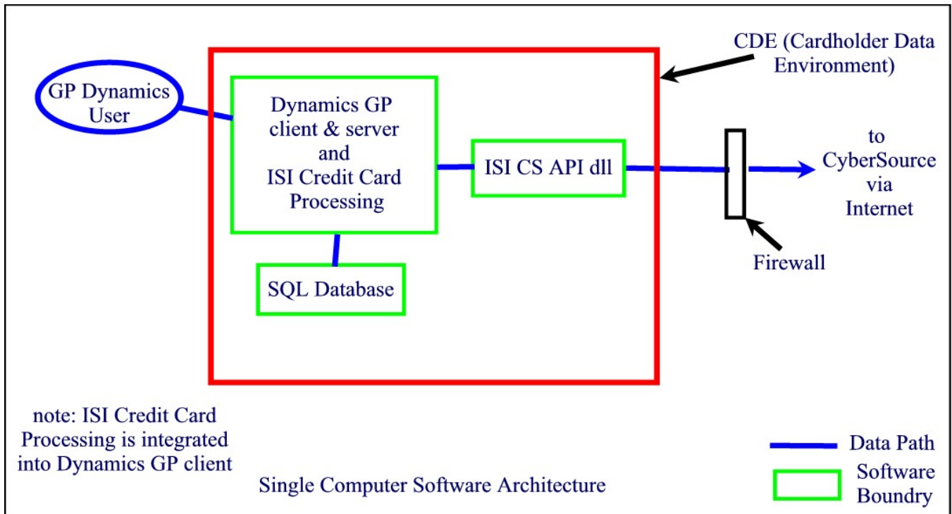
Diagram shows PCI Validated configuration using CyberSource
